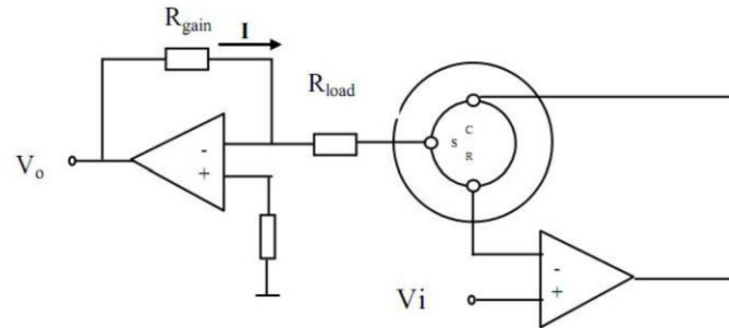
Basic Test Circuit for the SX-GVOCTSA Series Sensor
