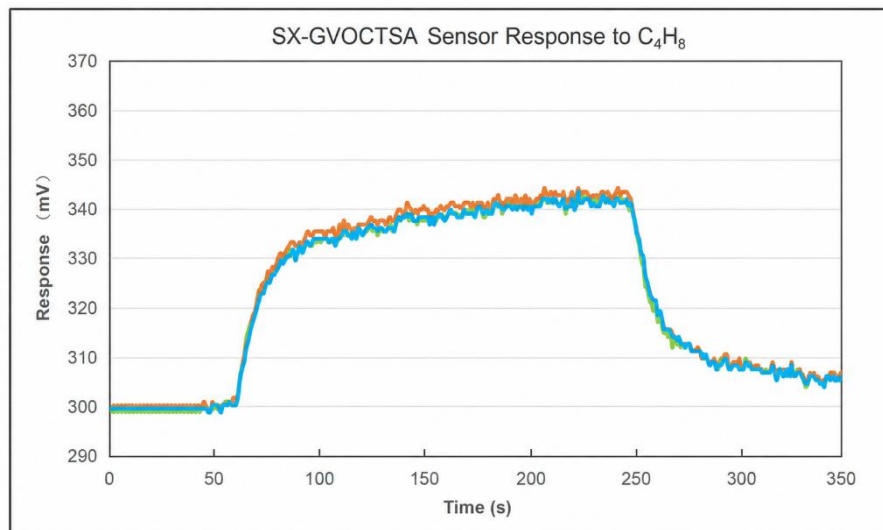
SX-GVOCTSA Sensor Response to C_4H_8 (Isobutylene)
