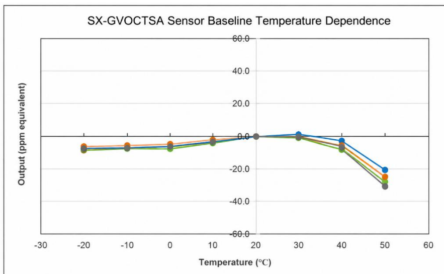
SX-GVOCTSA Sensor Baseline Temperature Dependence
