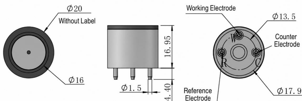
SX-GVOCTSA Sensor Dimensions
