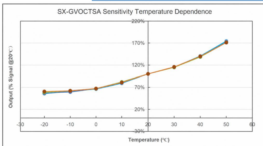
SX-GVOCTSA Sensor Sensitivity Temperature Dependence
