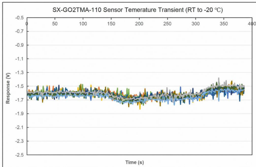
SX-GO2TMA Sensor Temperature Transient (Room Temp. to -20°C)
