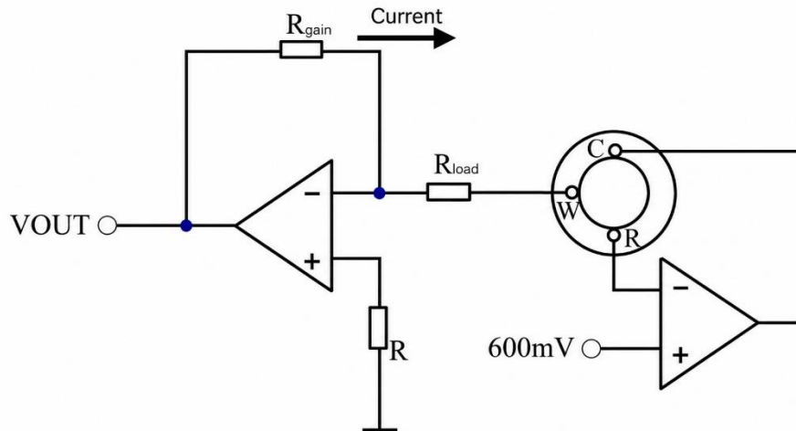
Recommended Circuit for the SX-GO2TMA Series Sensor
