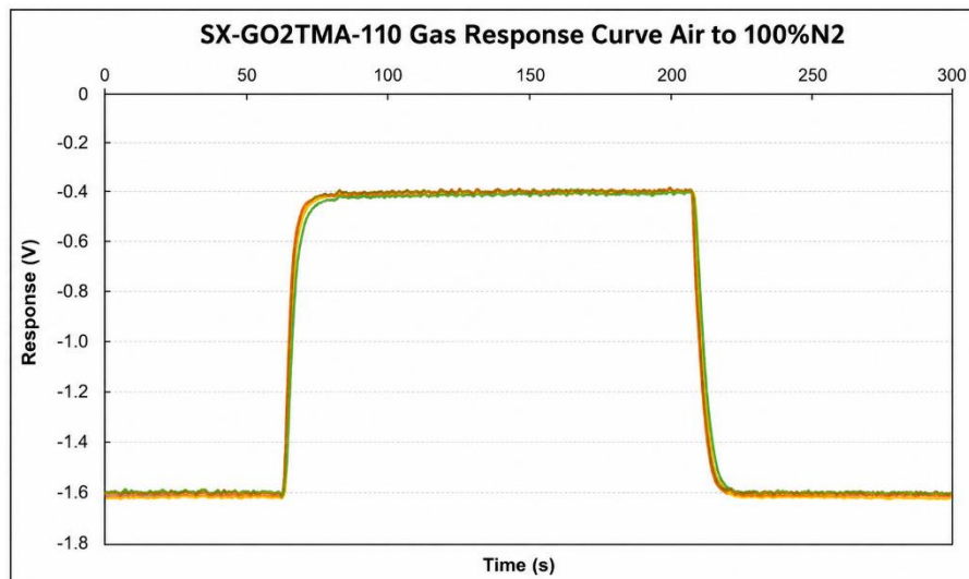
SX-GO2TMA-25% Gas Response Curve, Air to 100% N 2
