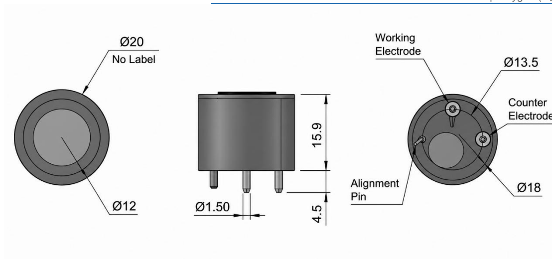
SX-GO2EGA Sensor Dimensions
