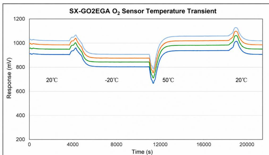
SX-GO2EGA O 2 Sensor Temperature Transient
