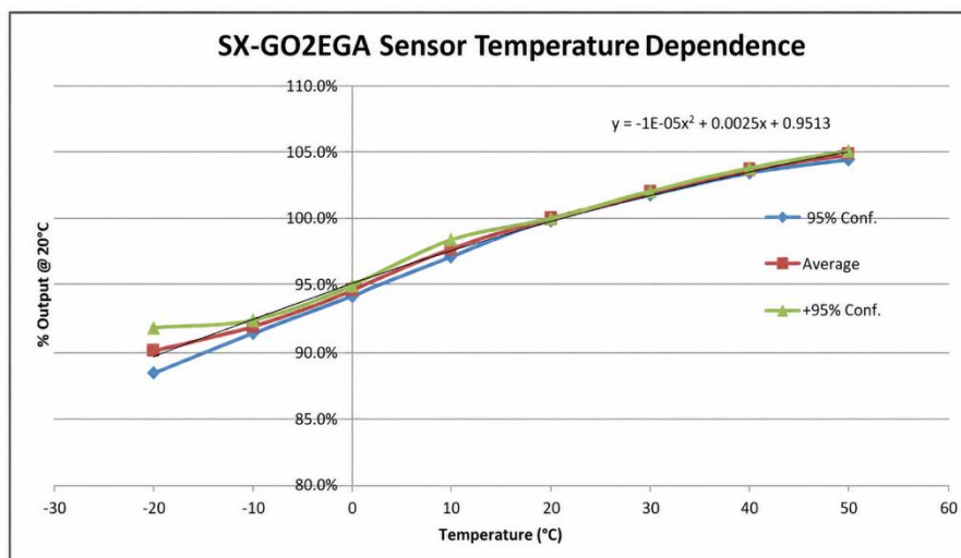
SX-GO2EGA Sensor Temperature Dependence
