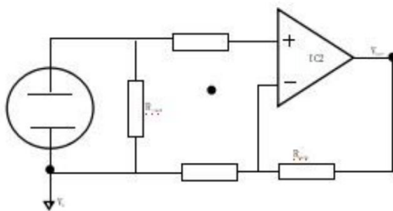
Recommended Circuit for the SX-GO2EGA Series Sensor
