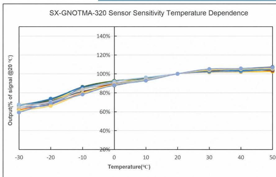
SX-GNOTMA Sensor Sensitivity Temperature Dependence
