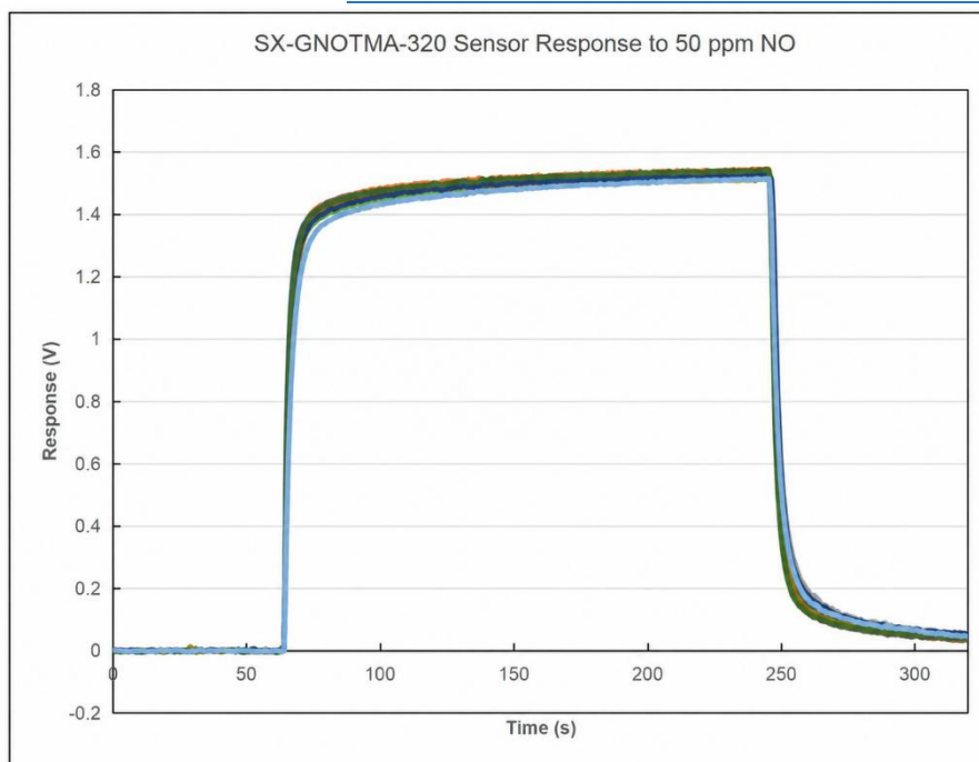
SX-GNOTMA Sensor Response to 50 ppm NO
