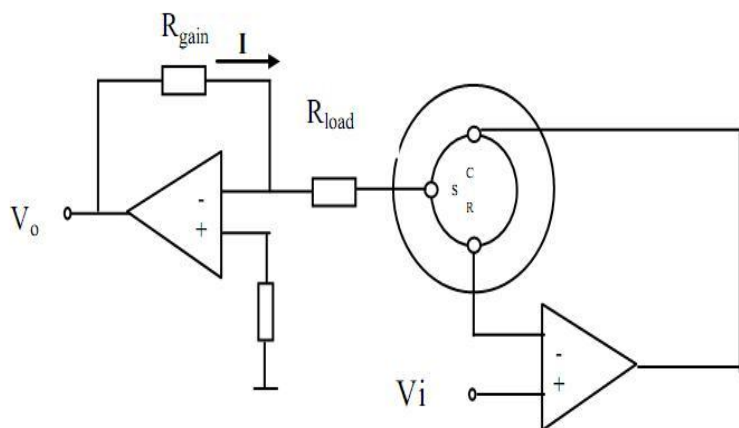
Basic Test Circuit for the SX-GNOTMA Series Sensor
