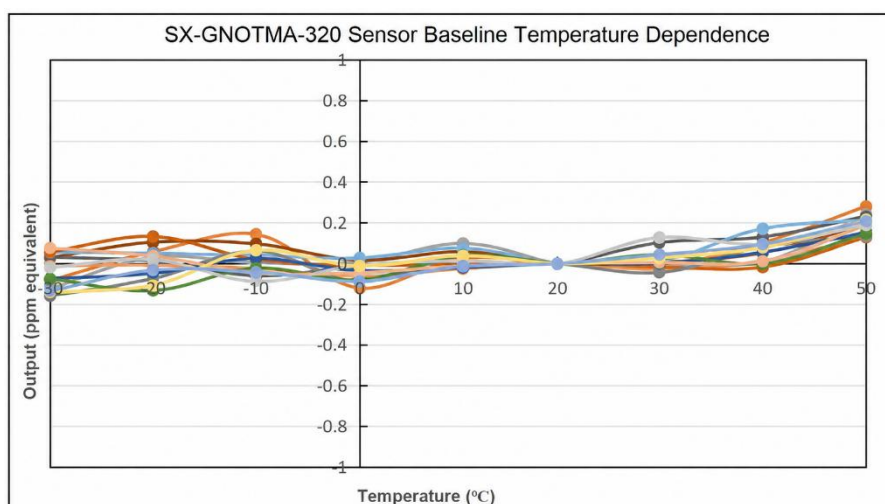
SX-GNOTMA Sensor Baseline Temperature Dependence
